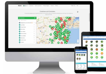
Software Hydrowise™
